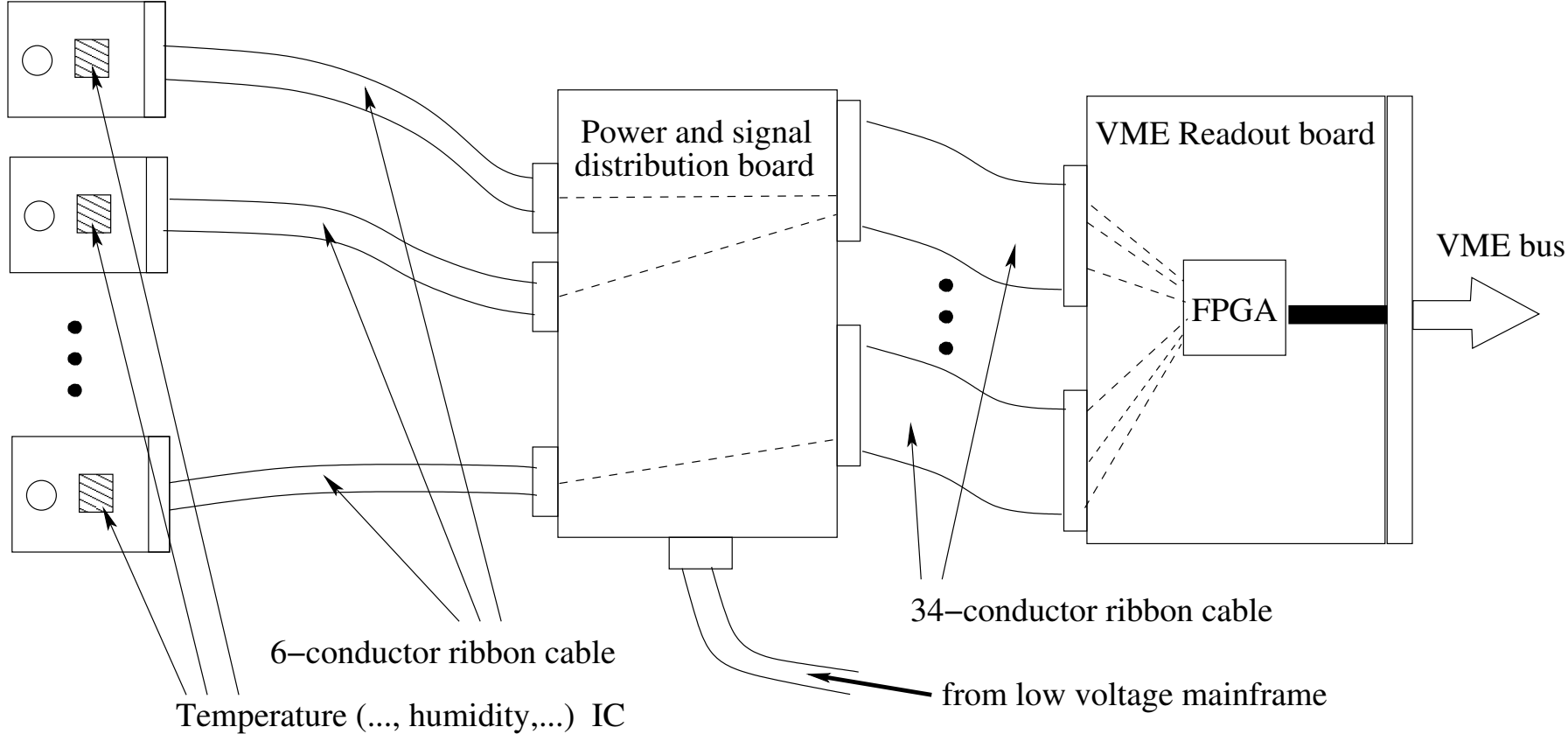
Slow control/sensor signal distribution and readout system
